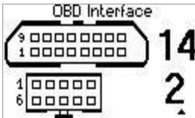
Fig. 2.3.4 Sample connection between STAG-OBd Adapter and CAN bus (2 of 2)
