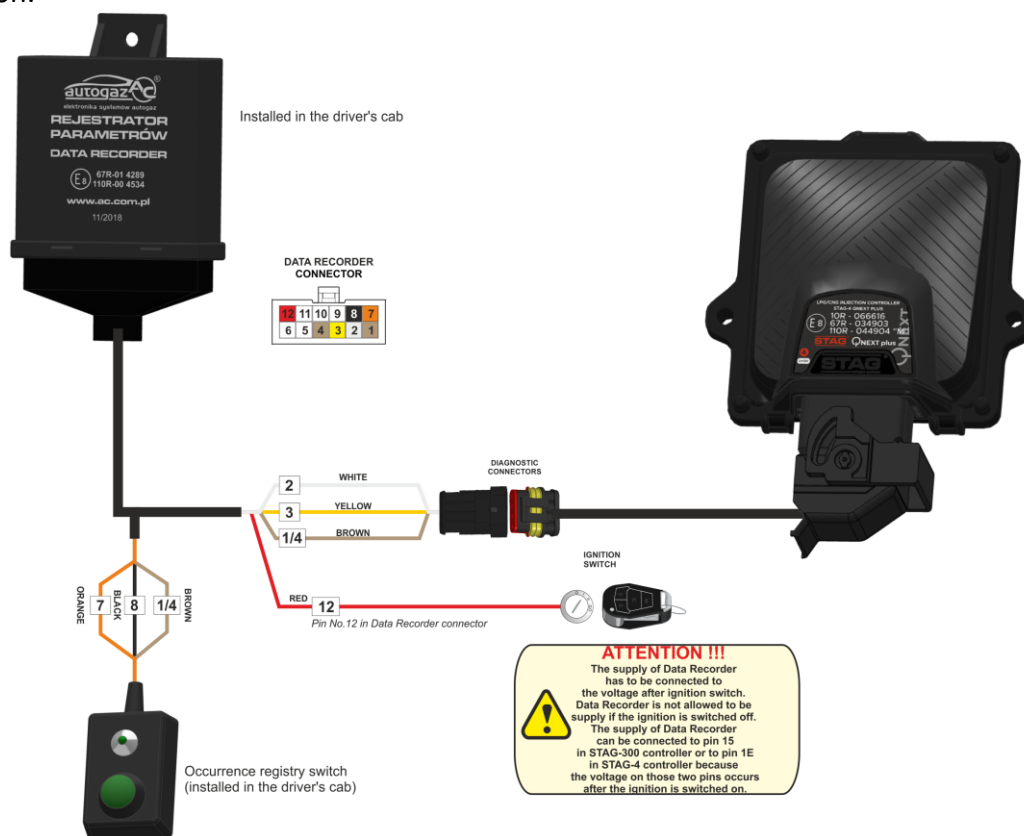
Fig. 1 Data Recorder Connection Diagram for Vehicle Installation.
